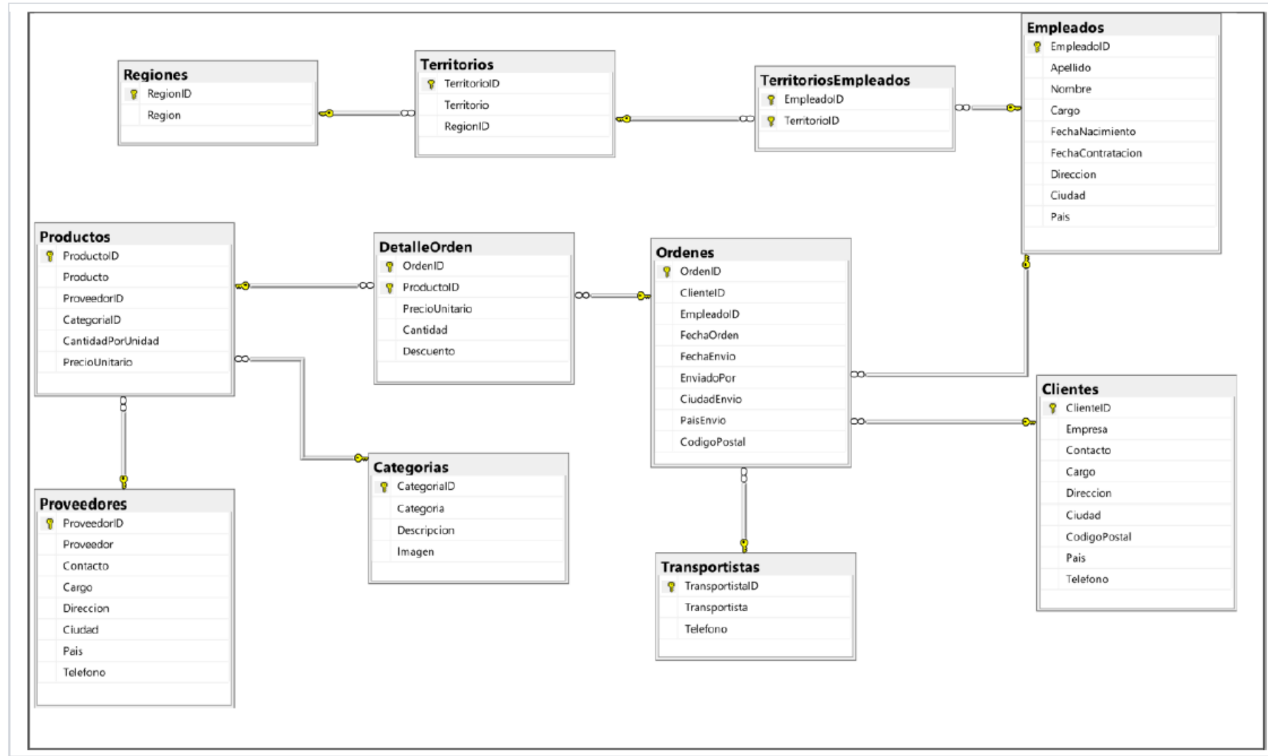
(Figura1): Modelo Relacional Kent Foods.
